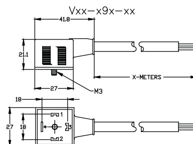
3 POLES + GROUND (GROUND OPPOSITE CABLE SIDE)
