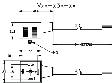
3 POLES + GROUND (GROUND CABLE SIDE)
