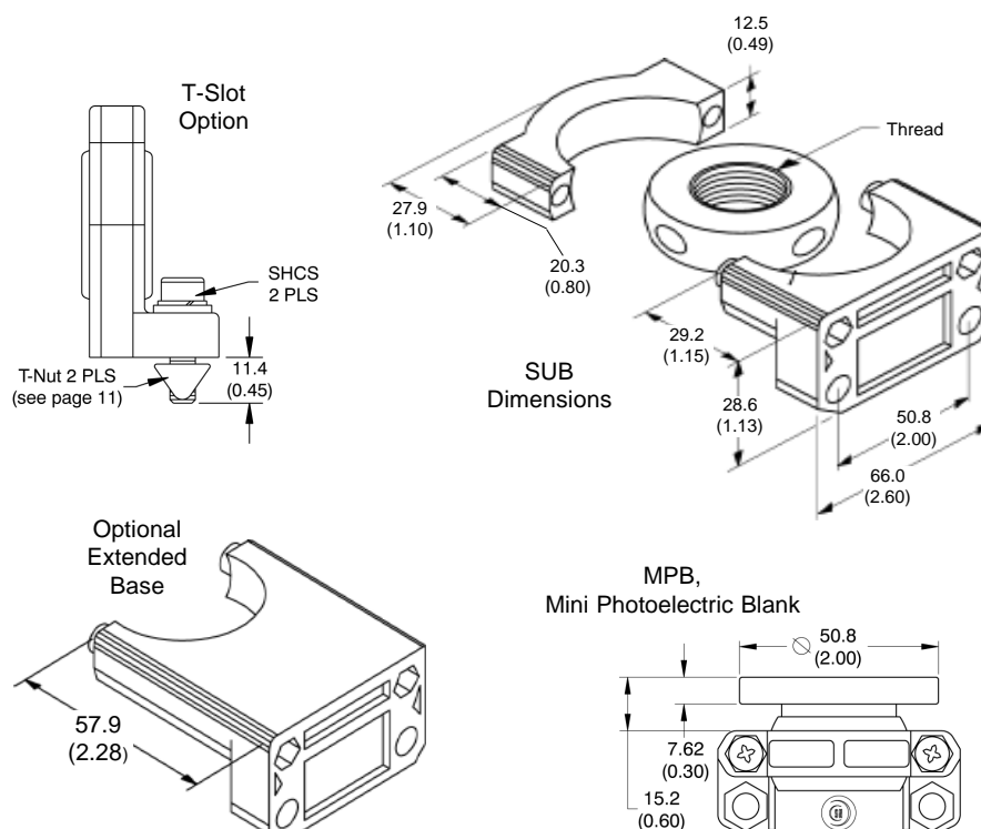
SUB-30 with photoelectric having a M30 x 1.5 threaded base.
