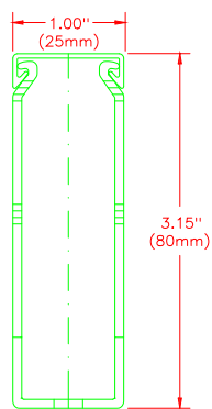
FRONT SECTION
