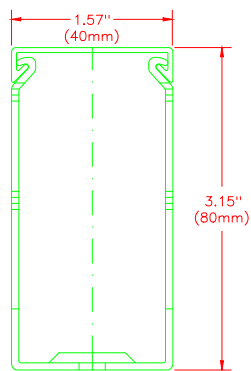
FRONT SECTION
