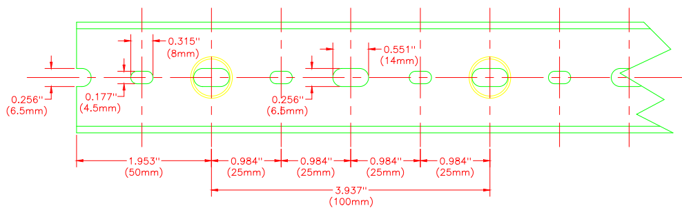
BASE PERFORATION
