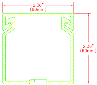
FRONT SECTION
