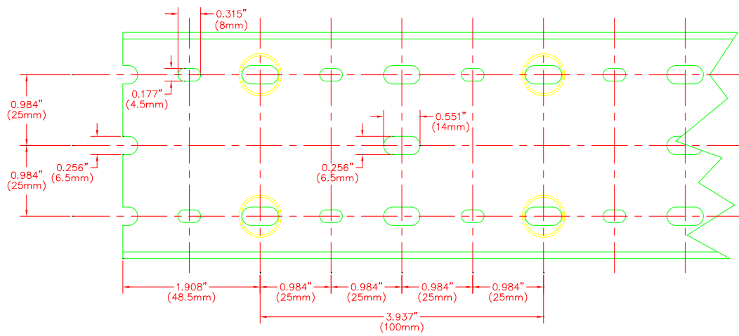
BASE PERFORATION
