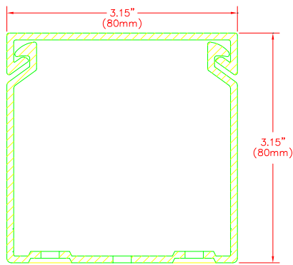
FRONT SECTION
